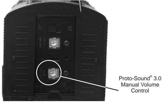
Figure 7: Manual Volume Control
