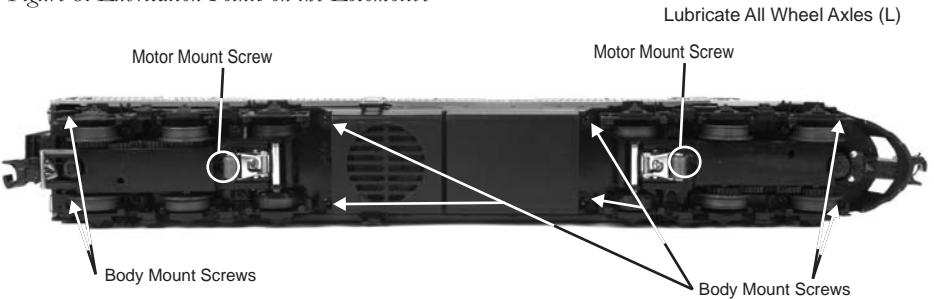
Figure 9: Body Mount Screws
