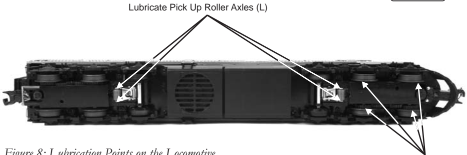
Figure 8: Lubrication Points on the Locomotive
