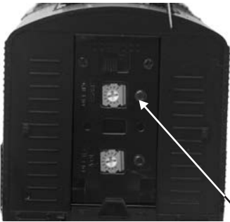
Figure 3: Controls Location [ Smoke and Volume Potentiometers ]
