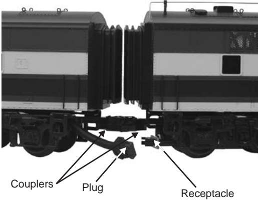
Figure 4: Connecting ABA Units
