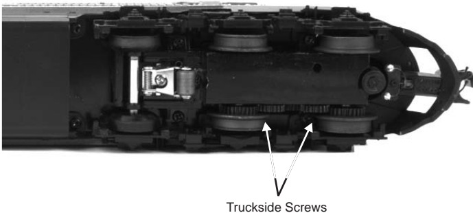
Figure 13: Truckside Screws
