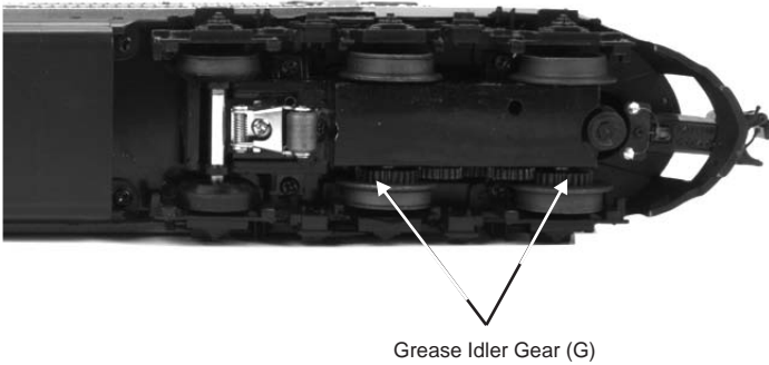
Figure 12: Greasing the Idler Gears
