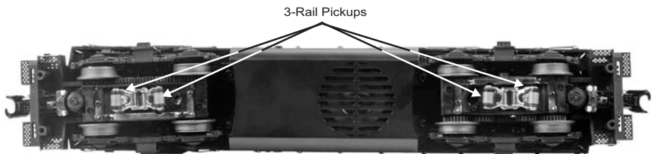
Figure 5: 2-Rail/3-Rail Operation
