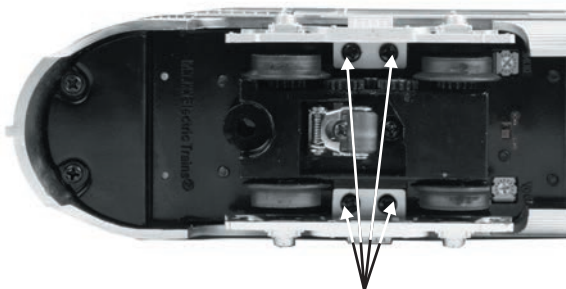
Figure 10: Truckside Screws
