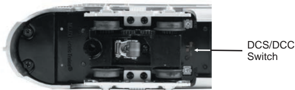
Figure 4: Changing from DCS to DCC Mode
