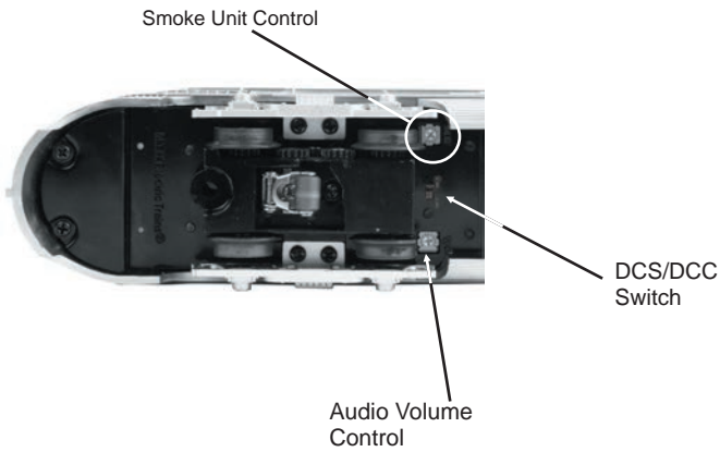
Figure 3: Smoke and Audio Unit Control
