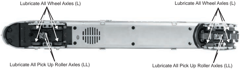
Figure 7: Lubrication Points on the Locomotive
