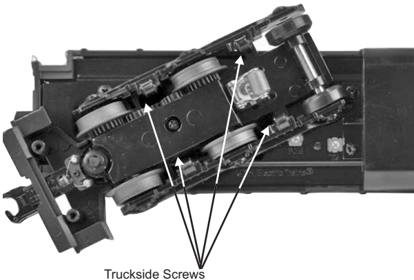
Figure 9: Truckside Screws
