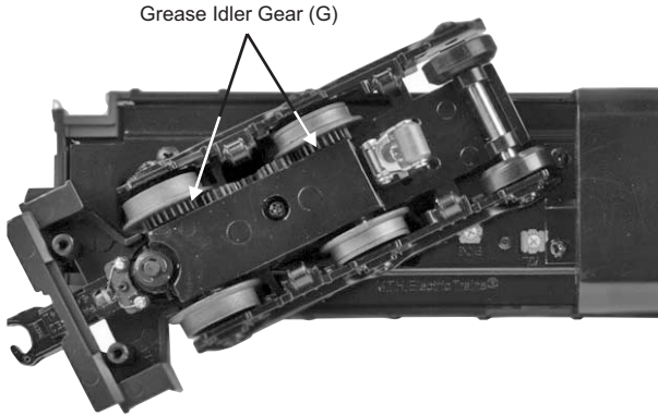
Figure 8: Greasing the Idler Gears
