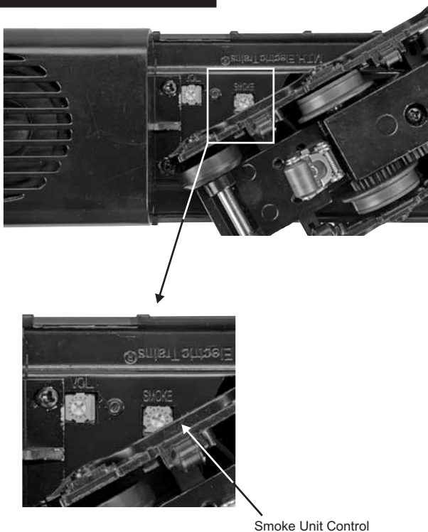
Figure 3: Smoke Unit Control
