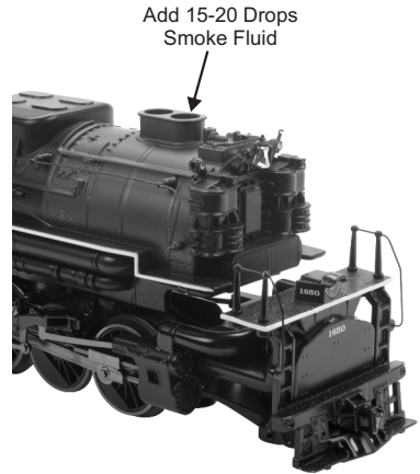
Figure 10: Adding Fluid
