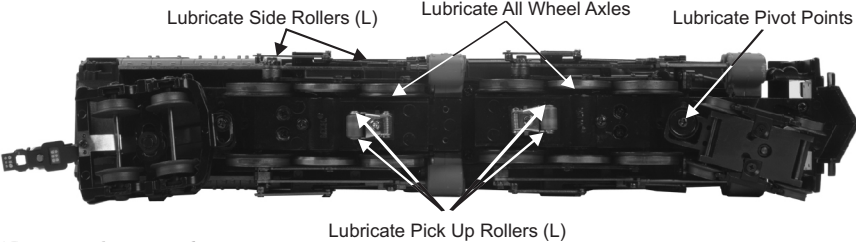
Fig. 8: Lubricating the Locomotive
