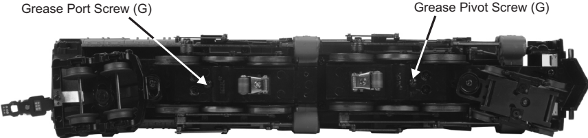
Fig. 9: Grease Points
