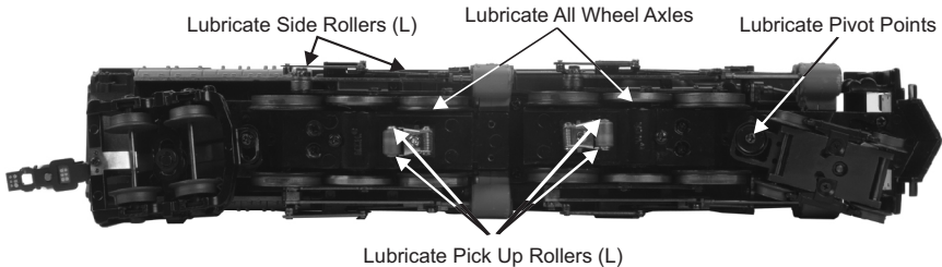
Fig. 1: Lubricating the Locomotive
