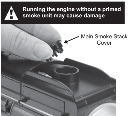
Figure: Remove Smoke Stack Cover
