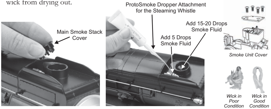
Figure: Remove Smoke Stack Cover
