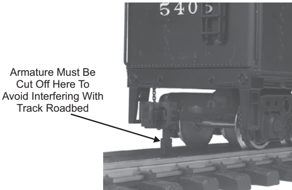
Figure: Standard Knuckle Coupler in Position "B"
