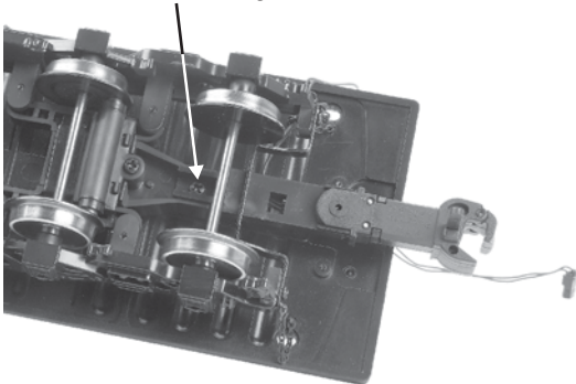
Figure: Coupler Armature Mounting Screw
