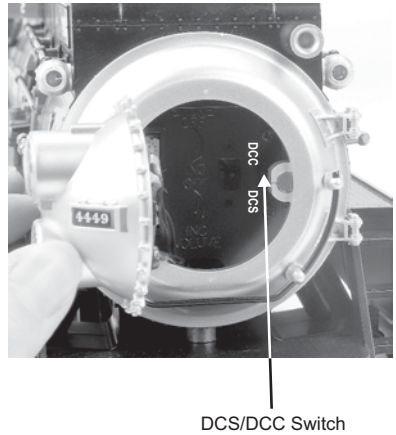
Figure: Changing from DCS to DCC Mode
