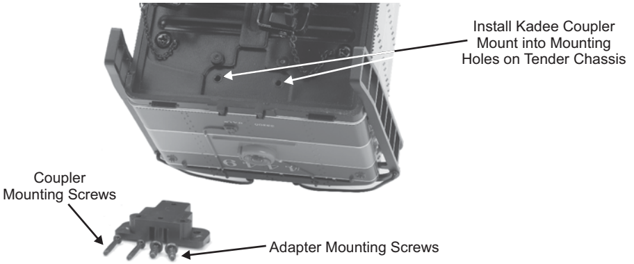
Figure: Kadee Coupler Adapter Plate
