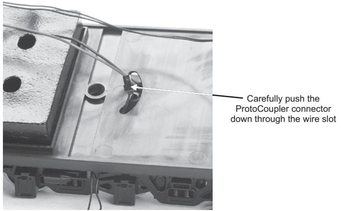
Figure: Removing the ProtoCoupler connector
