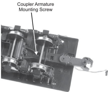
Figure: Removing the coupler armature mounting screw
