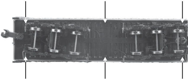
Figure: Body Mount Screw Locations
