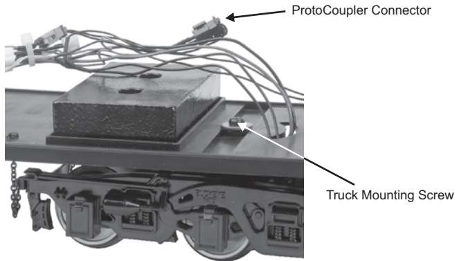
Figure: ProtoCoupler Connector and Truck Mounting Screw
