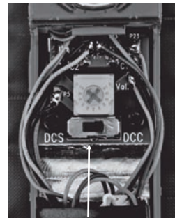
DCC-DCS switch
