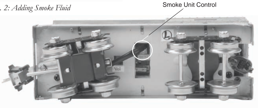
Fig. 3: Smoke Unit Control
