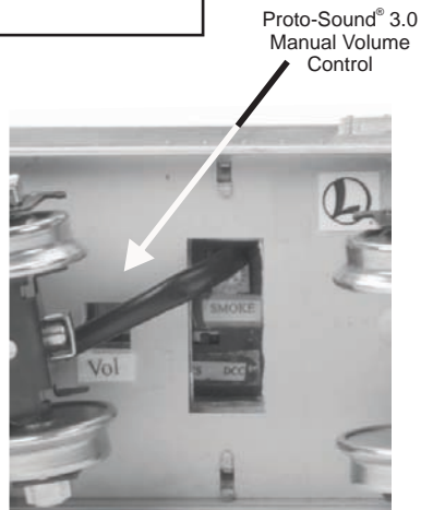
Fig. 7: Manual Volume Control
