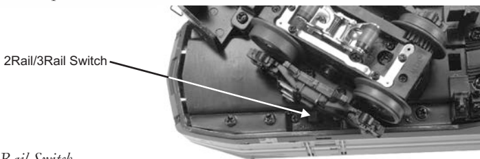
Figure: 2Rail/ 3Rail Switch
