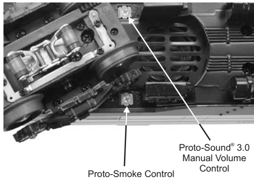
Figure: Manual Volume Control/Smoke Volume Control
