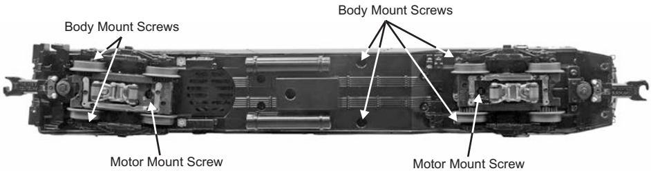
Figure: Body Mount Screws
