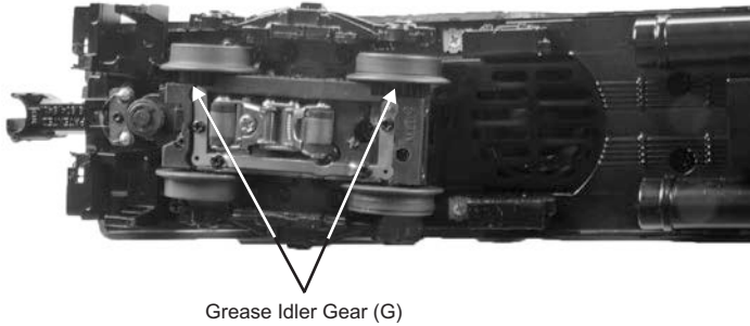
Figure: Greasing the Idler Gears
