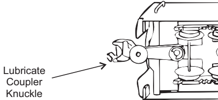
Figure 3: Lubricating The ProtoCouplers
