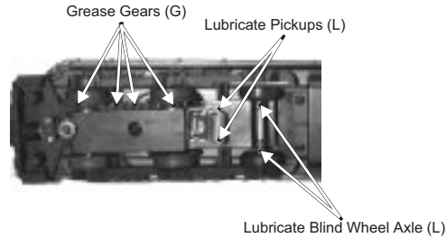
Figure 6: Lubricating The Locomotive Chassis
