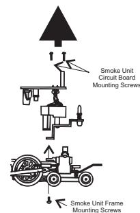
Figure 2: Inspecting The Smoke Unit
