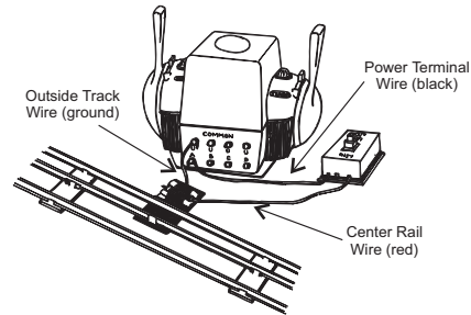
Figure 5: Wiring Up A Bell Button
