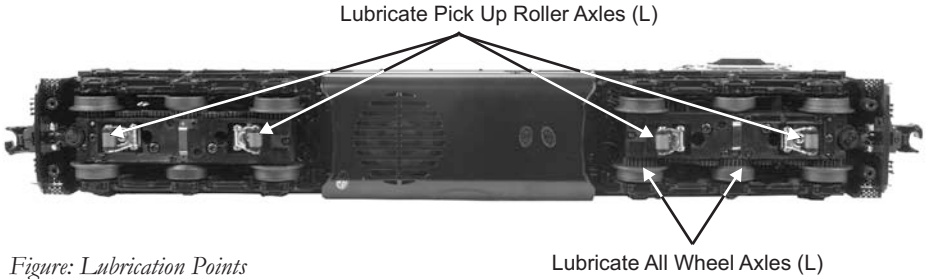
Figure: Lubrication Points
