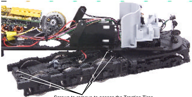
Screws to remove to access the Traction Tires Figure 8. Locations of Truckside Mounting Screws
