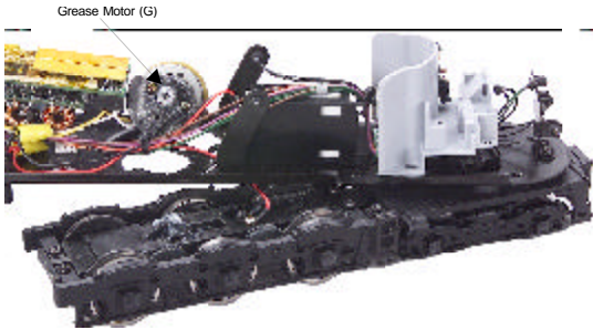
Figure 7. Greasing the Worm Gear on the Motor
