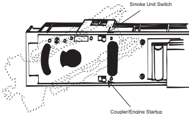
Figure 1: Locating The Smoke Unit Switch
