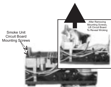
Figure 2: Inspecting The Smoke Unit
