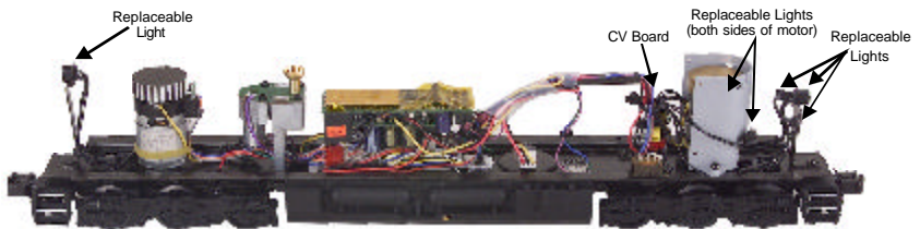
Figure 9. Replacing the Lights in your Engine
