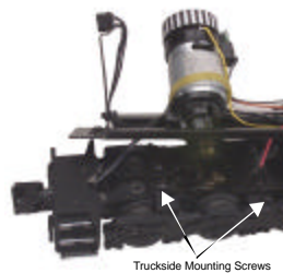
Figure 8. Truckside Mounting Screws to Access the Traction Tires
