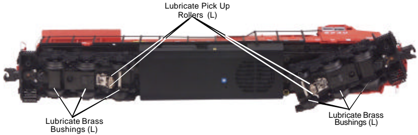
Figure 5. Lubrication Points on the Locomotive
