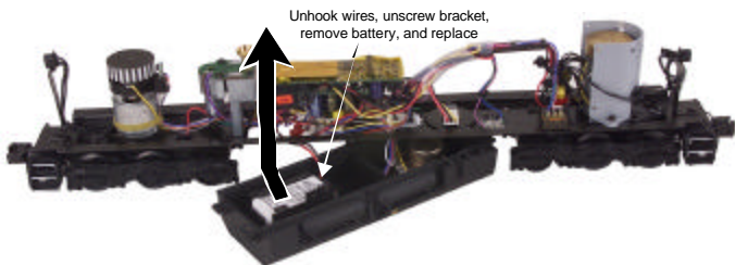
Figure 11. Replacing the Battery (Remove the remaining 2 screws on the fuel tank to access the battery.)
