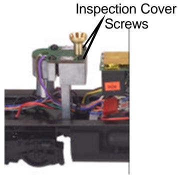
Figure 4. Inspecting the Smoke Unit
