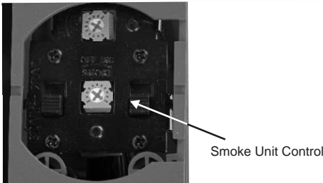
Figure 3: Accessing Smoke Unit Control
