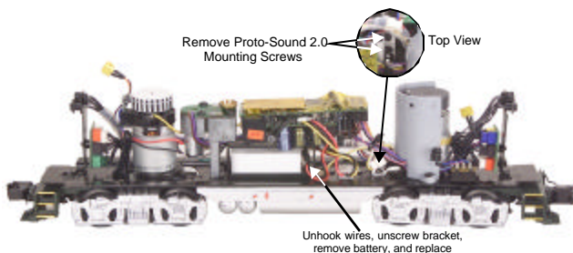
Figure 11. Replacing the Battery (Remove the Proto-Sound 2.0 Board to access the battery.)
