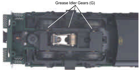
Figure 6: Greasing The Idler Gears
