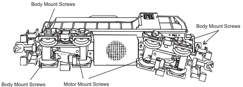
Figure 7: Removing the locomotive chassis
