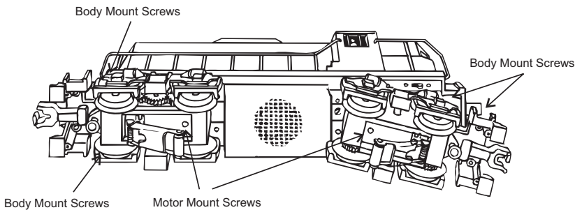
Figure 8: Removing The Body From The Chassis
