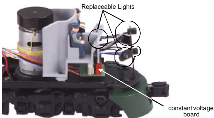
Figure 9. Locations of Replacable Lights
