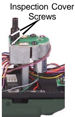
Figure 5. Inspecting the Smoke Unit
