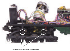
Figure 8. Locations of Truckside Mounting Screws
