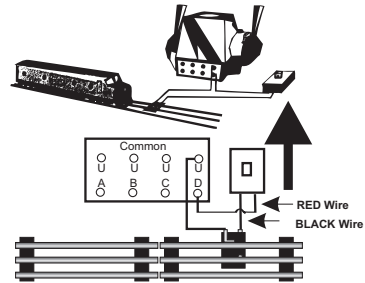
Figure 6: Wiring Up A Bell Button
