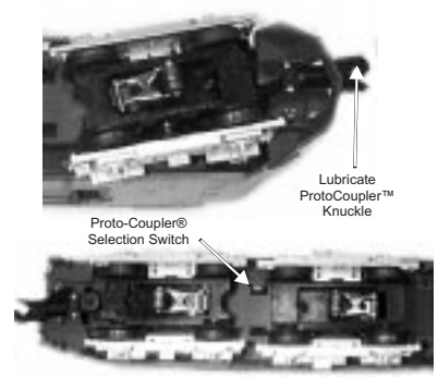
Figure 5: Locating the ProtoCoupler Switches and Lubricating The ProtoCouples
