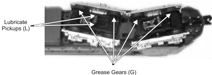
Figure 6: Lubricating The Locomotive Chassis
