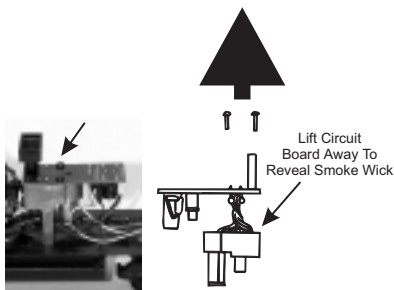
Figure 4: Inspecting The Smoke Unit
