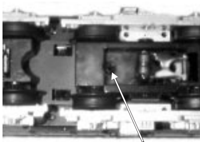
Figure 7: Lubricate The Tender Chassis Trucks
