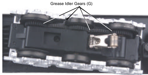
Figure 4 : Greasing the gears
