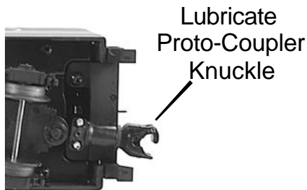
Figure 5: Lubricating The ProtoCoupler
