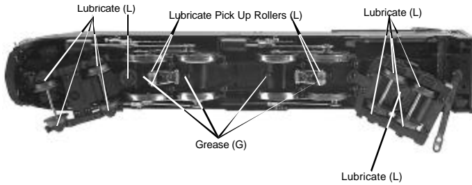
Figure 8: Lubricating The Locomotive Chassis
