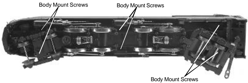
Figure 10: Removing The Boiler From The Chassis
