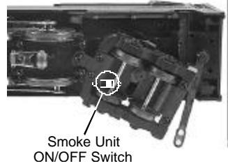
Figure 3: Smoke Unit Switch (under trailing truck)
