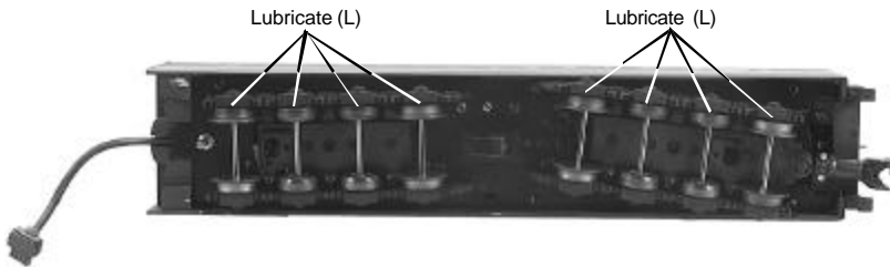
Figure 9: Lubricate The Tender Chassis Trucks
