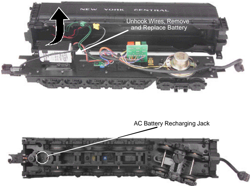
Figure 115: Replacing The Battery And Locating The Battery Recharging Jack
