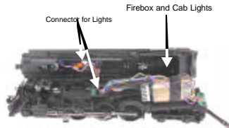
Figure 9: Boiler Connector Cables
