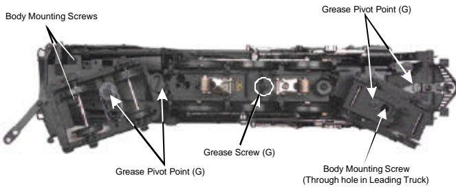
Figure 6: Removing The Body
