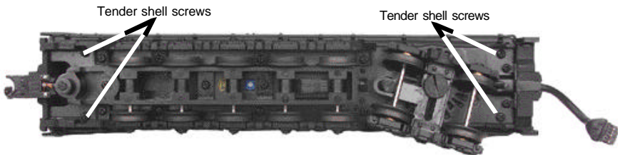
Figure 10: Removing The Tender Body
