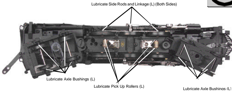
Figure 5: Lubricating The Chassis
