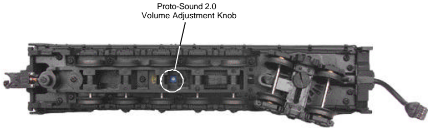
Figure 4: Manual Volume Adjustment
