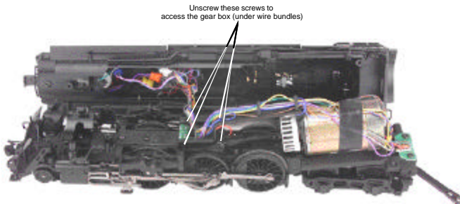
Figure 6: Opening The Gearbox
