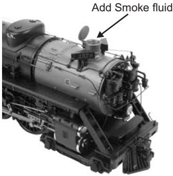
Figure 2: Adding Smoke Fluid
