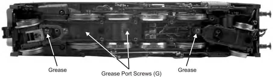
Figure: Grease Points
