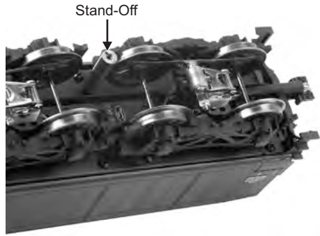
Figure: Remove the stand-offs from the engine and tender
