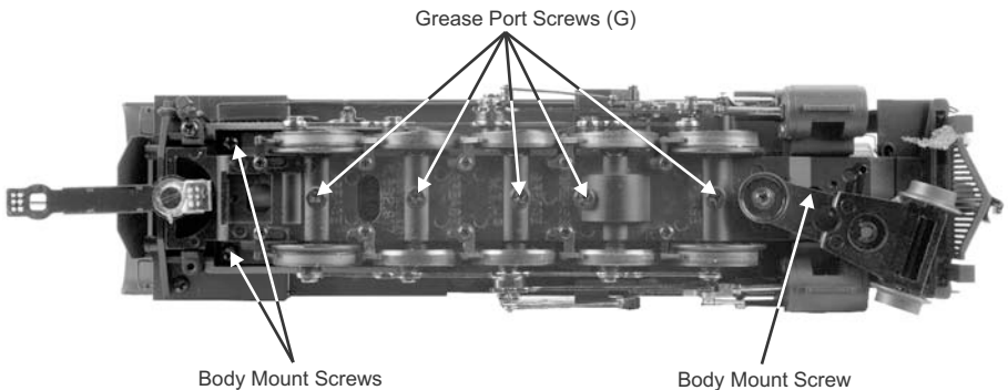
Figure: Grease Points & Body Mount Screw Locations
