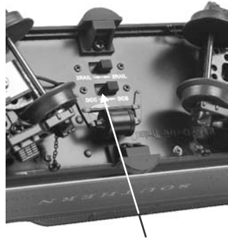
DCS/DCC Switch
