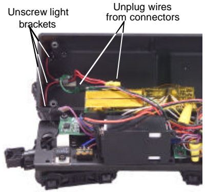
Figure 8. Changing the Tender Light.
