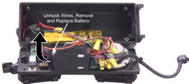
Figure 9. Replacing the Battery
