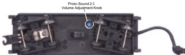
Figure 2. Manually Adjusting the Proto-Sound 2.0 Volume
