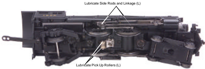
Figure 6. Lubrication Points on the Locomotive
