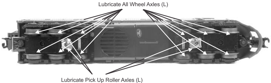
Figure: Lubrication Points on the Locomotive
