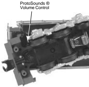
Figure 4: Adjusting The ProtoSound Volume and selecting the ProtoCoupler™
