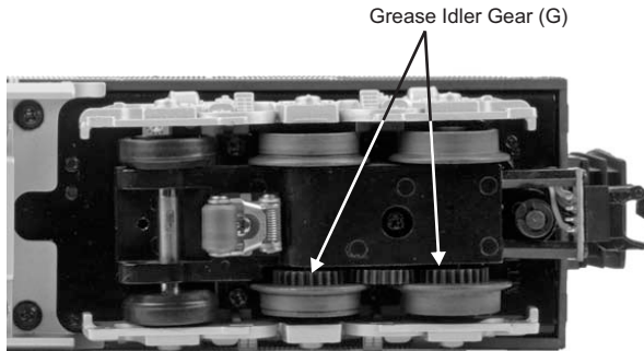
Figure 8: Greasing the Idler Gears
