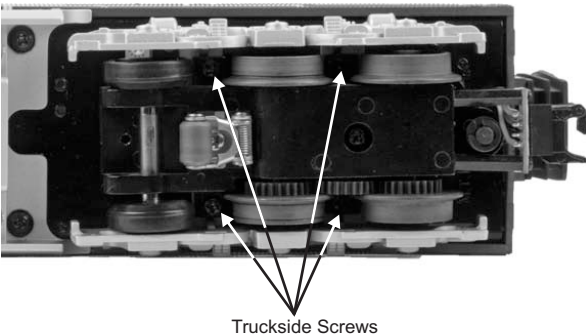
Figure 9: Truckside Screws
