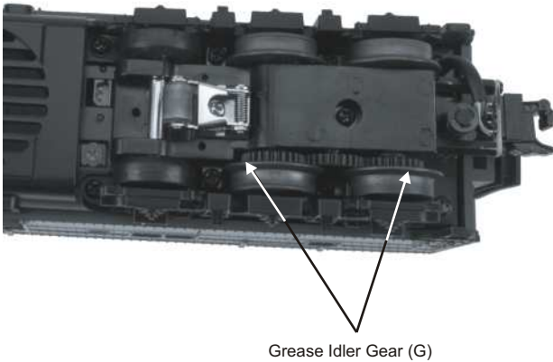
Figure 5. Greasing The Idler Gears
