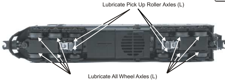
Figure 3. Lubrication Points on the Locomotive
