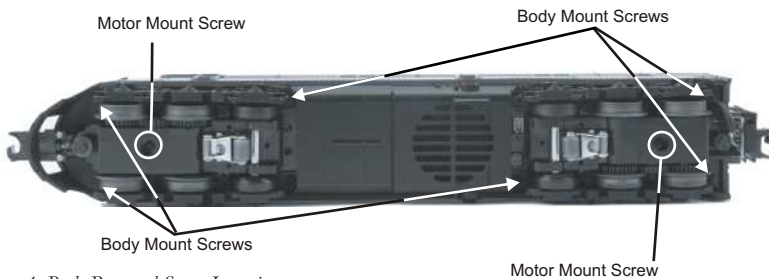
Figure 4. Body Removal Screw Locations
