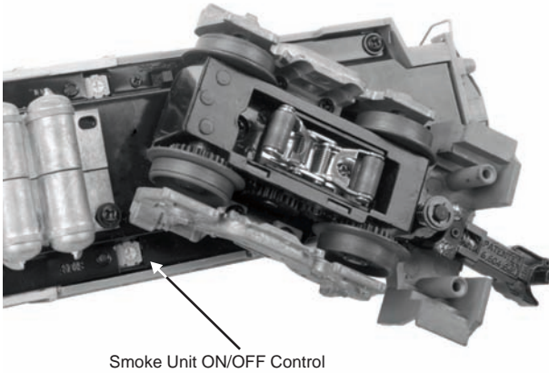
Figure 3. Smoke Unit Control
