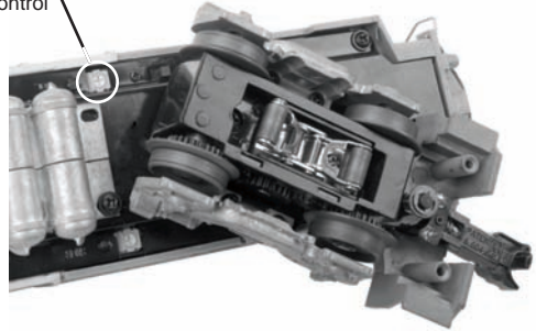
Figure 5: Manual Volume Control
