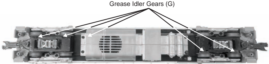
Figure 8: Greasing The Idler Gears
