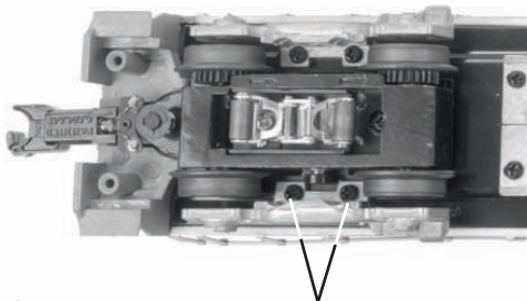
Truckside Screws
