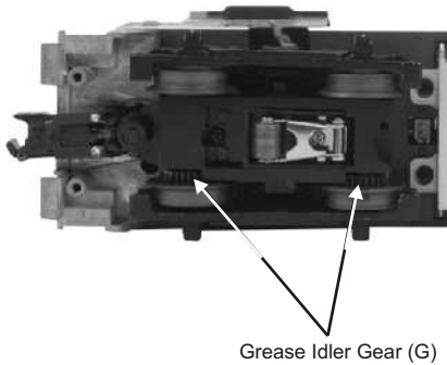
Figure 6. Greasing The Idler Gears
