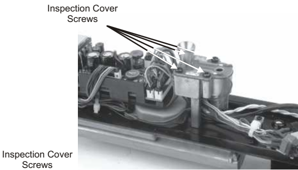
Figure 8. Inspecting the Smoke Unit Wick
