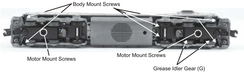
Figure 5. Body Removal Screw Locations
