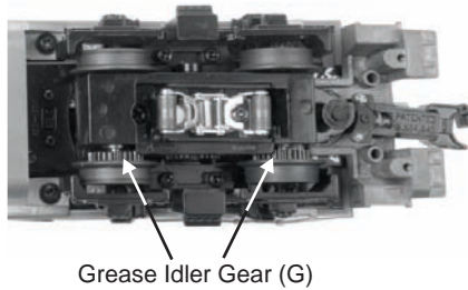
Figure 8: Greasing The Idler Gears
