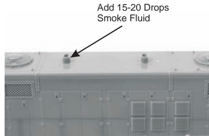
Fig. 10: Adding Fluid
