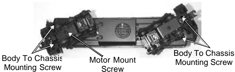
Figure 7: Removing The Locomotive Chassis
