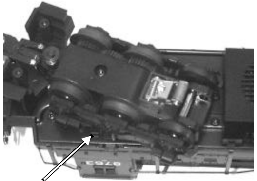
ProtoCoupler™ Selection Switch
