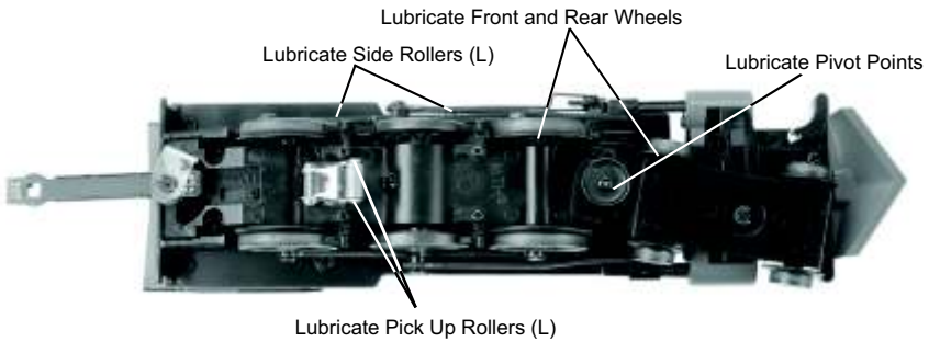
Fig. 8: Lubricating the Locomotive
