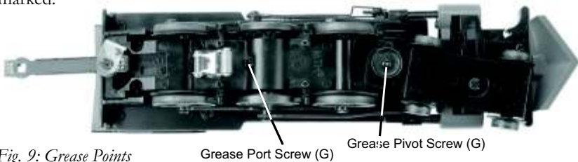
Fig. 9: Grease Points
