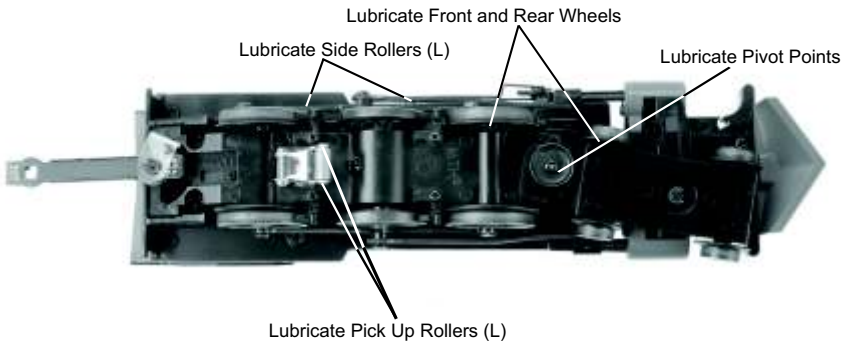
Fig. 1: Lubricating the Locomotive
