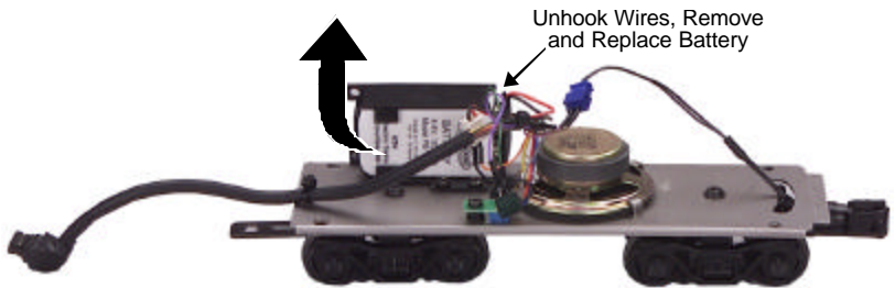
Figure 9. Replacing the Battery
