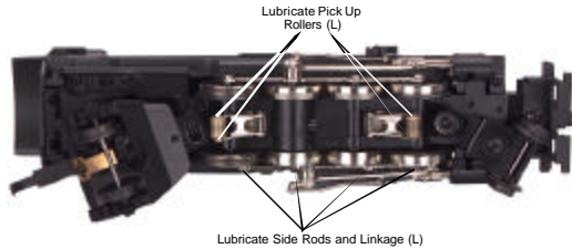
Figure 2. Lubrication Points on the Engine
