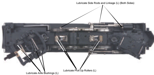
Figure 1. Lubrication Points on the Locomotive
