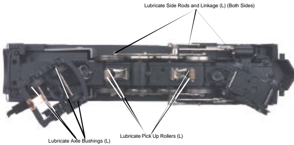
Figure 5: Lubricating the Locomotive
