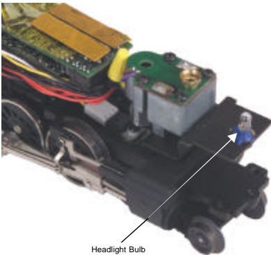
Figure 7: Headlight Location
