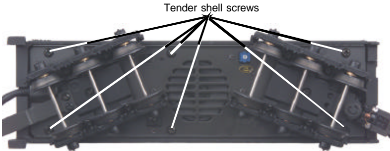
Figure 8: Removing The Tender Body
