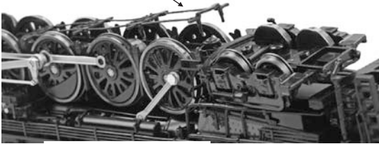
Brake Shoe Lever & Bellcrank
